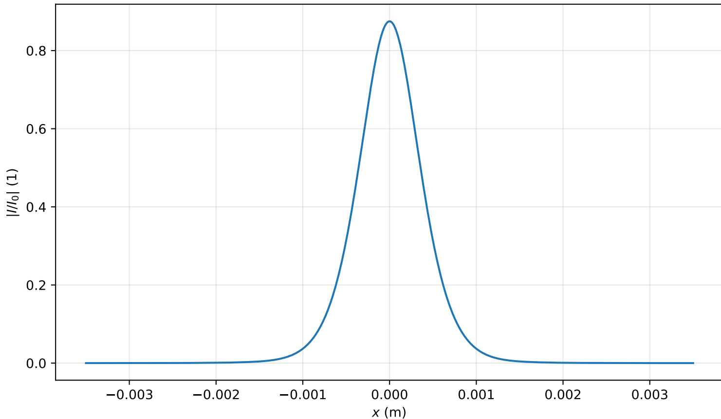
Intensity profile I(x, y = 0, z = 2.866m)/I_0 , P_{in}=0.7P_{cr} , artificial time
